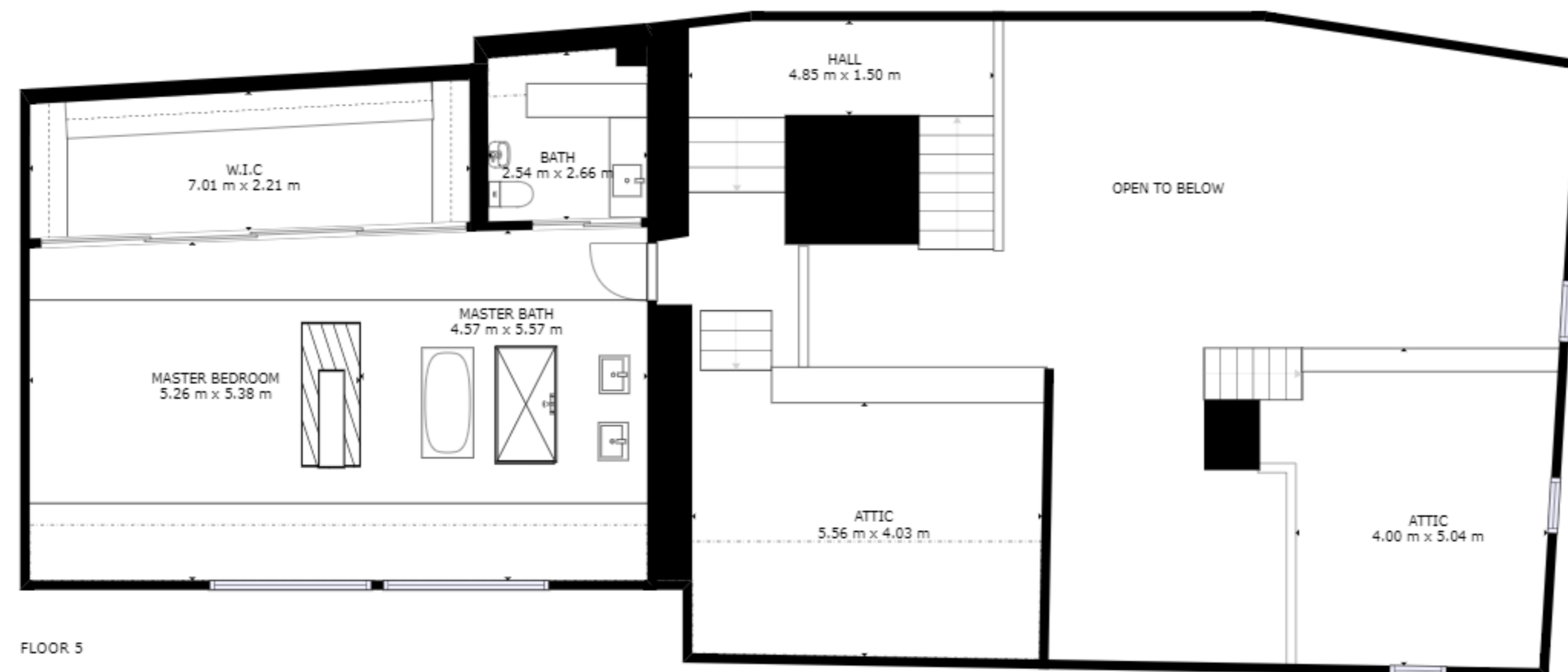
FLOOR 5
