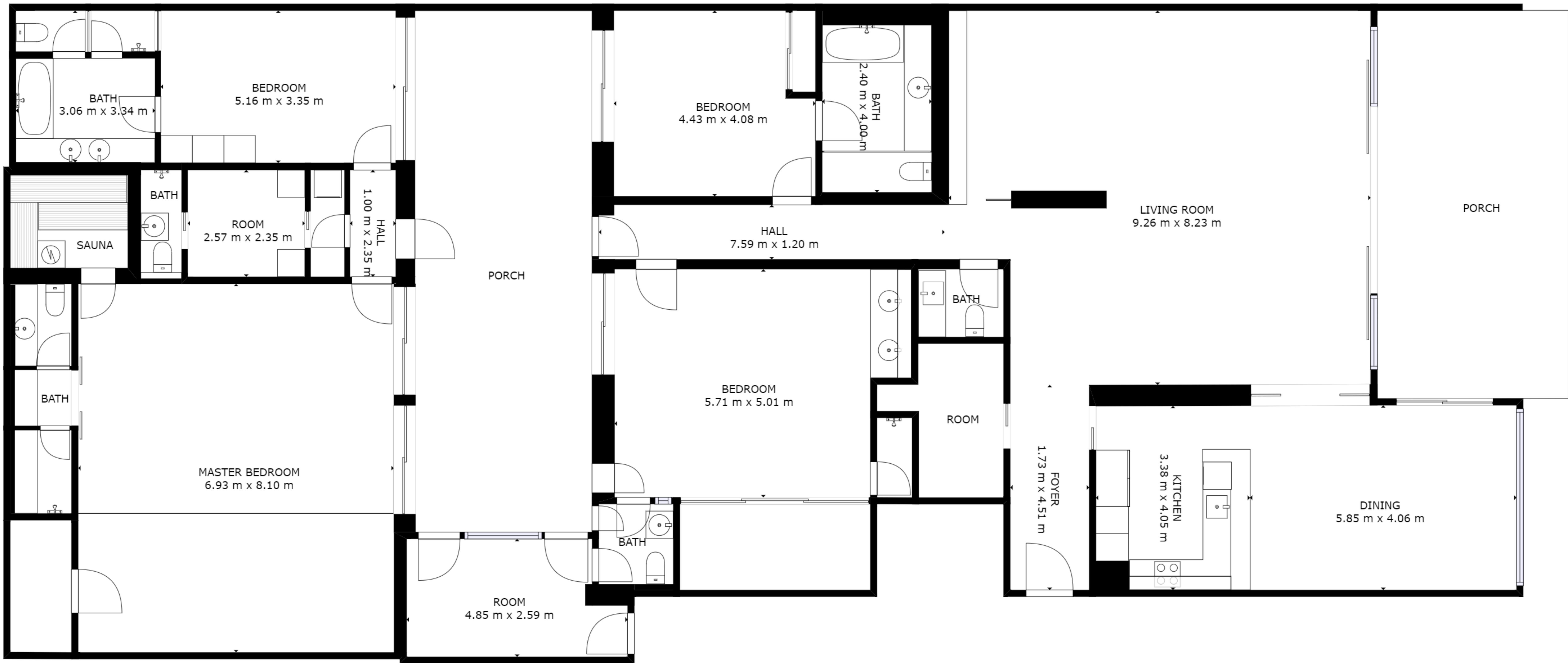
FLOOR 1
